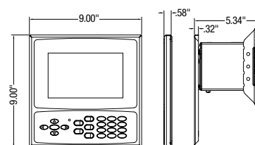
Panel Mount
