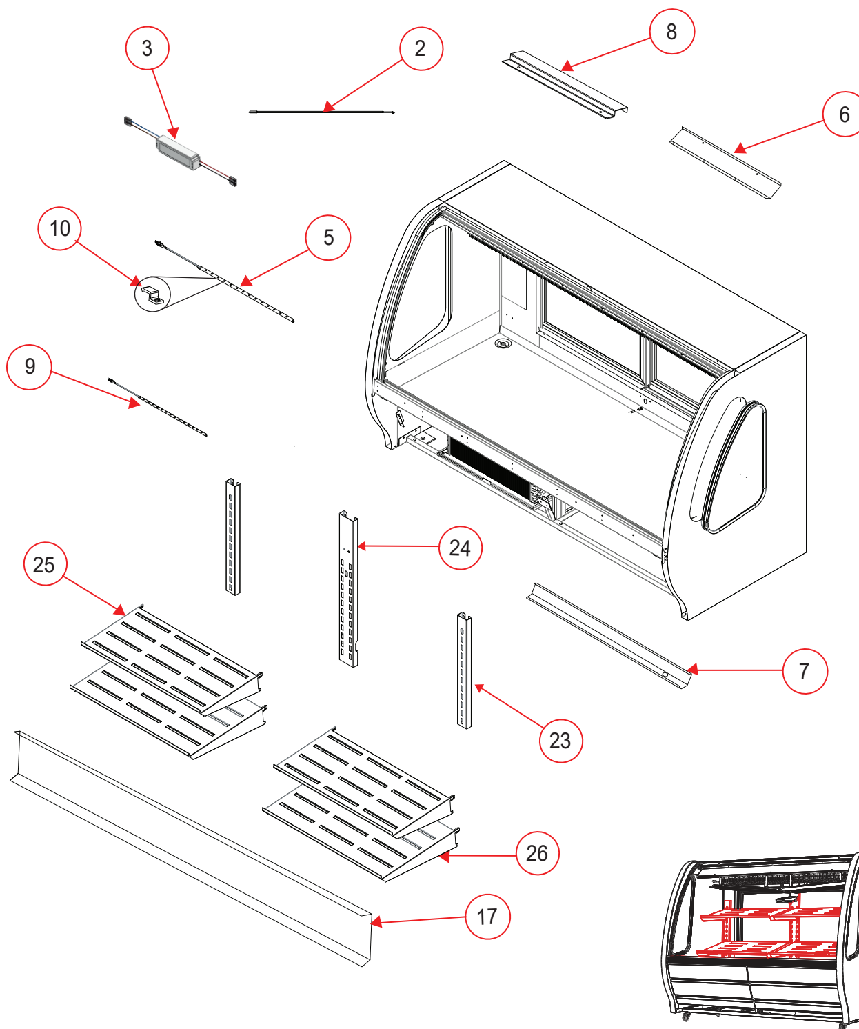
ENSAMBLE GENERAL INTERIOR
