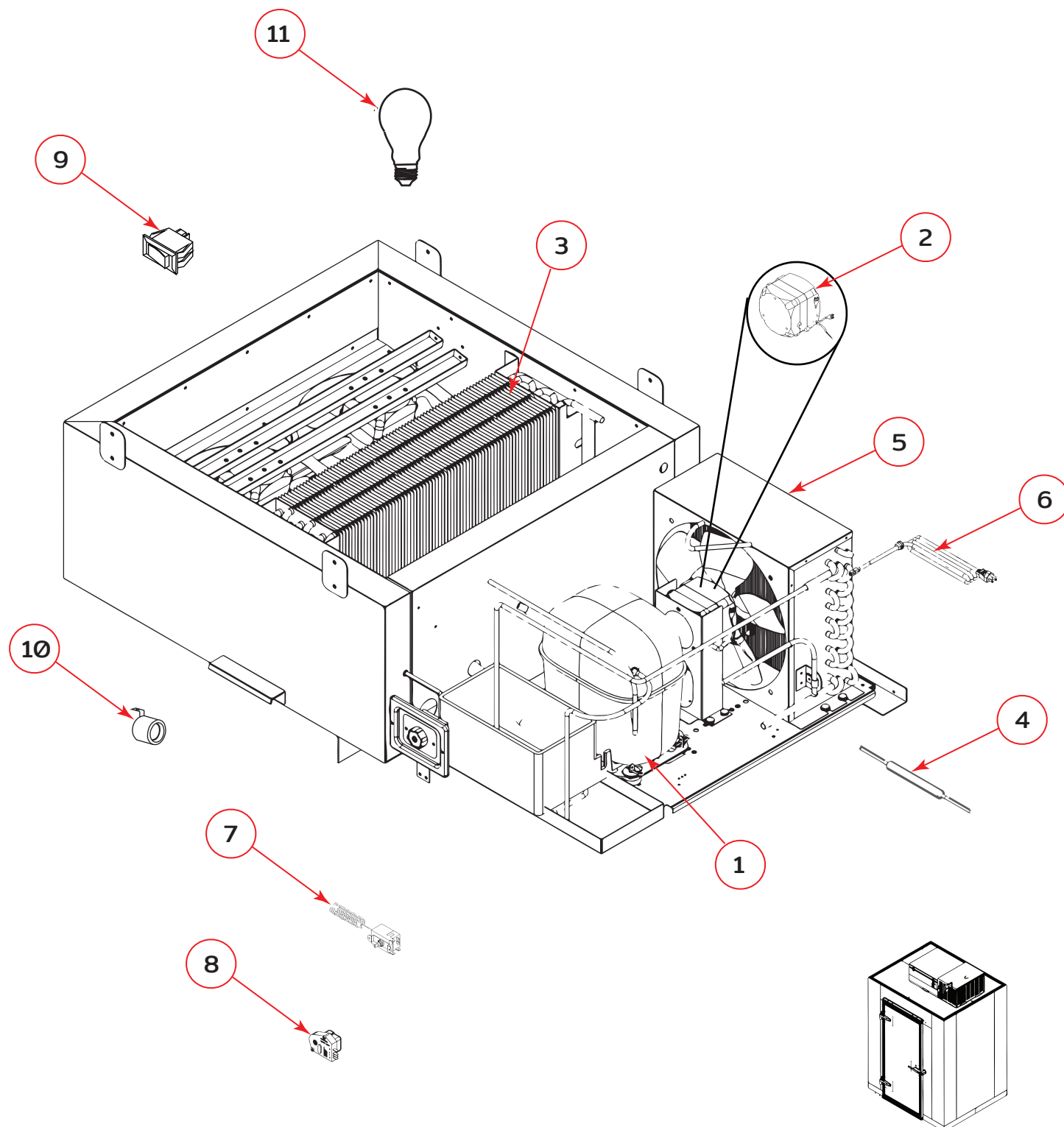
ENSAMBLE GENERAL
