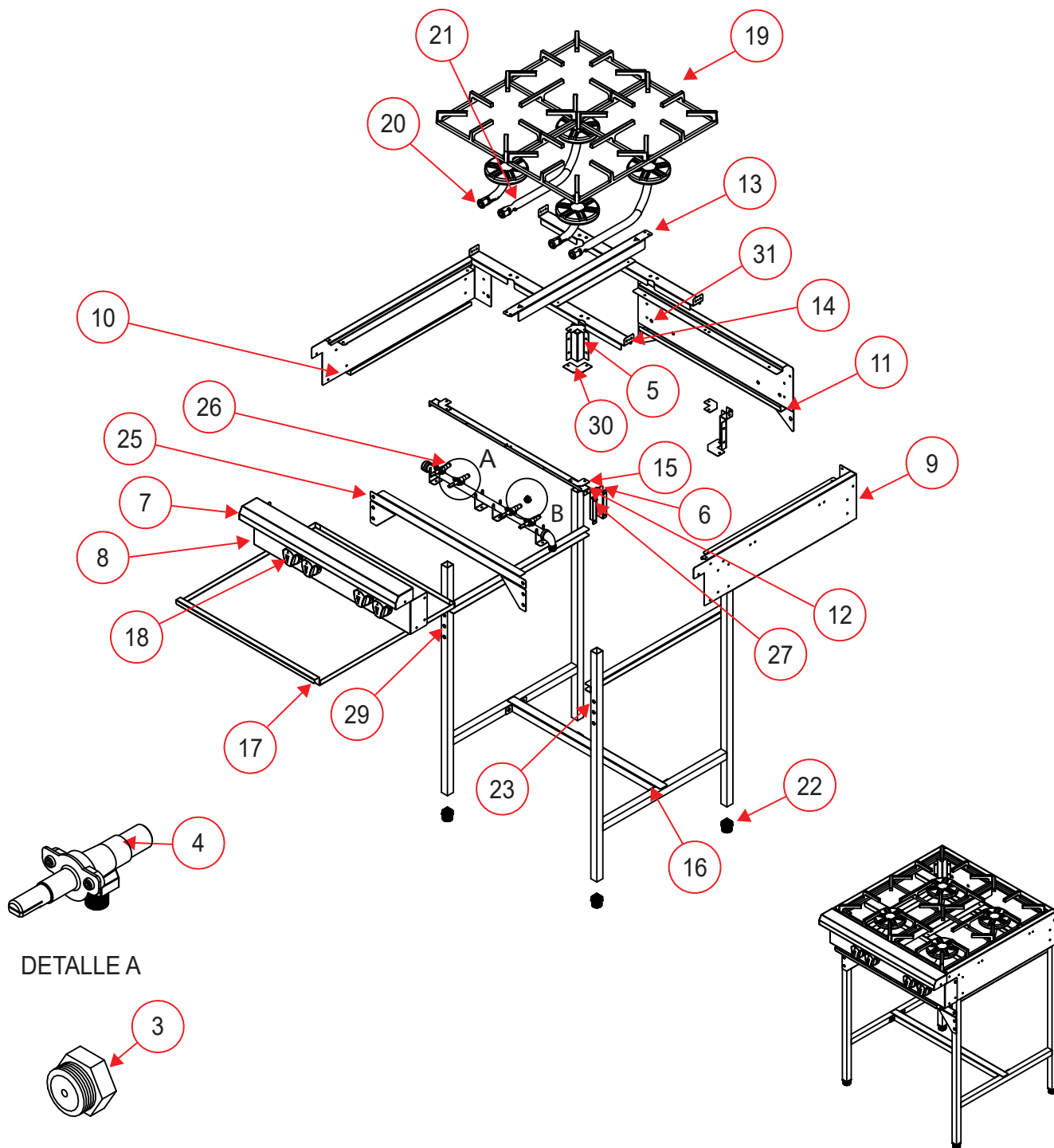
ENSAMBLE GENERAL EXTERIOR
