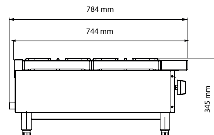
LATERAL
